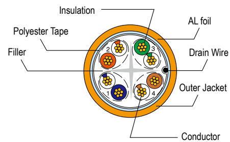
Cross section
