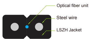
FCS11-1-S Cable Structure
