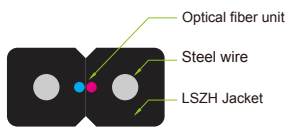
FCS11-2-S Cable Structure
