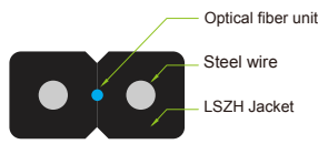
FCM11-1-S Cable Structure
