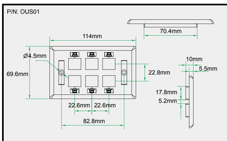
Six ports USA faceplate
